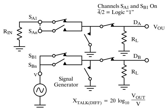
Figure 10. Differential Crosstalk
