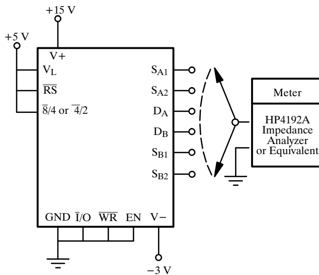
Figure 12. Off State Input/Output Capacitance
