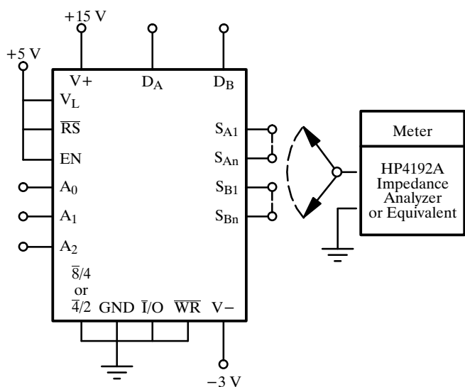
Figure 11. On State Input Capacitance
