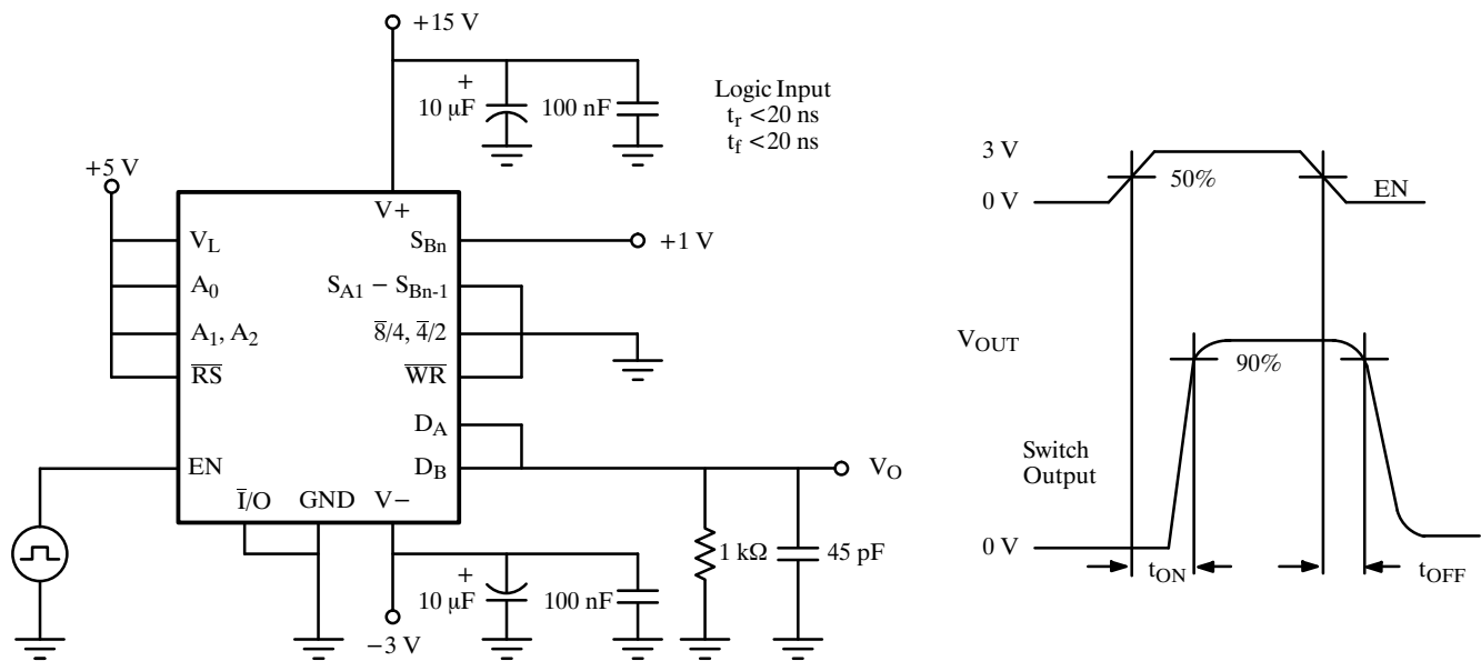
Figure 2. EN, CS, \overline{CS} , Turn On/Off Time
