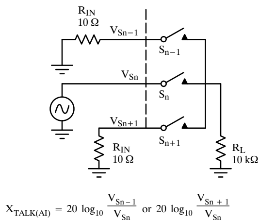
Figure 9. Adjacent Input Crosstalk
